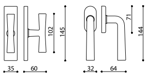
C105R - fixed window slider
